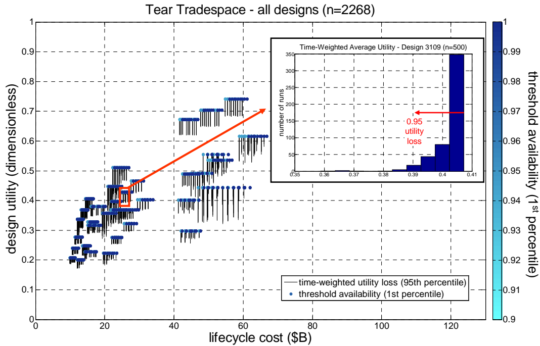
Figure 7 Survivability “tear” tradespace for a Satellite Radar System (Ref. 7)
