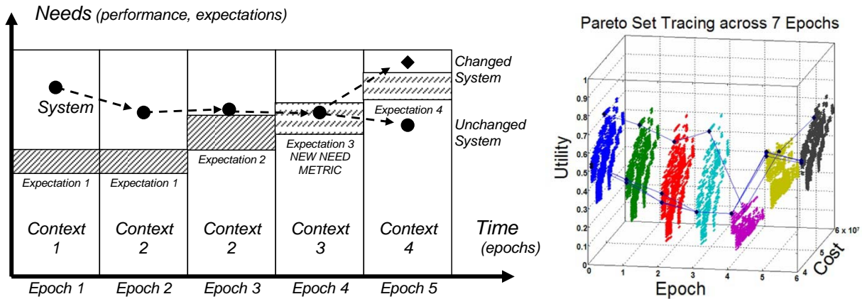
Figure 8 Epoch series representation for system timelines (l) and cross-epoch analysis for identifying “robust” designs in tradespaces (r)
