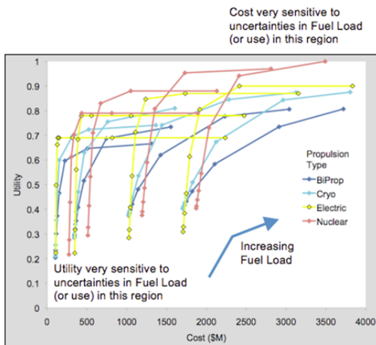
Figure 13. Sensitivity studies give insight into uncertainty issues
