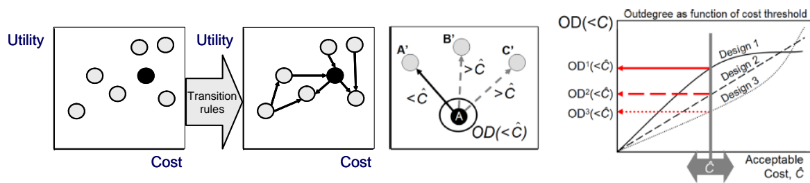
Figure 5 Tradespace network as tradespace with applied transition rules (l) (Ref. 4) and filtered outdegree as tradespace network-based changeability metric (r) (Ref. 16)
