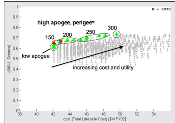
Figure 9. X-TOS tradespace initial exploration
