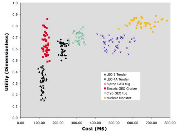
Figure 14. Monte Carlo simulation of general uncertainty in the Space Tug tradespace
