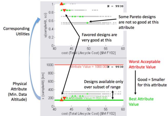
Figure 10. Min. Data Altitude attribute and its utility versus cost
