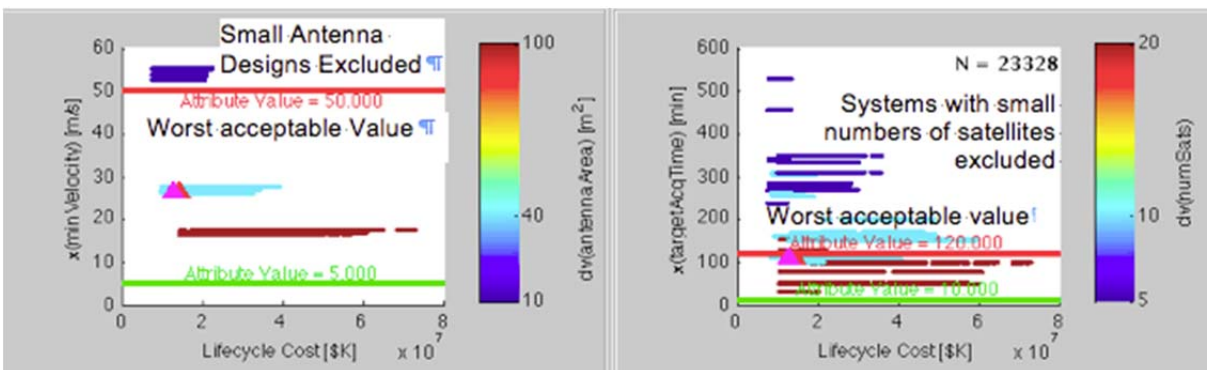
Figure 11 Attribute versus cost plots with limits included show designs eliminated from the tradespace
